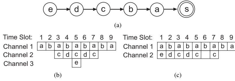
Fig. 14.7 (a) A line network with 5 source nodes. (b) Schedule length is 9 using 3 channels when nodes can buffer at most one packet. (c) Schedule length is 9 using 2 channels when nodes can buffer multiple packets.
