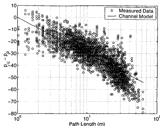
Figure 4. Measurements fit channel model
