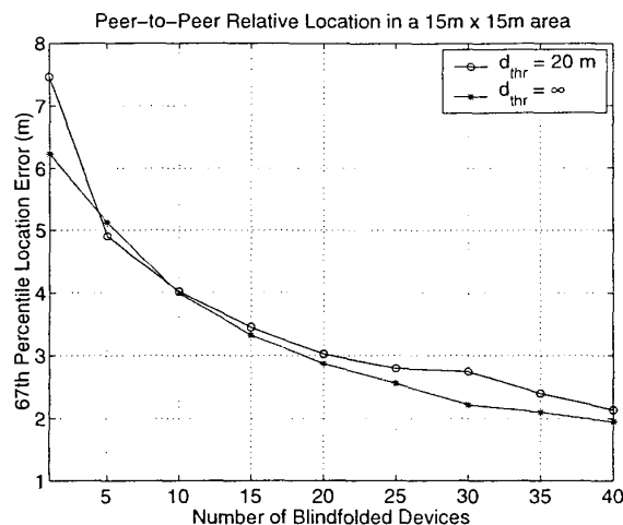
Figure 1. Simulated 67 th percentile errors
