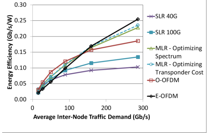
Fig. 6. Energy Efficiency achieved for different networking solutions as a function of the average inter-node traffic demand.
