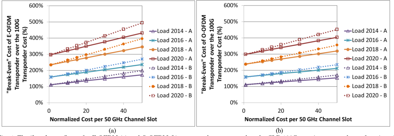
Fig. 4. The “break-even” cost for E-OFDM (a) and O-OFDM (b) transponders compared to the SLR 100G case is presented as a function of the normalized cost per 50 GHz channel slot under different traffic loads settings. Costs are normalized to the value of a 10G transponder. Options A (solid line) and B (broken line) correspond to a cost value for a 100G transponder of 5.5 and 3.75 cost units respectively. The additional cost of a flex-grid OXC over a fixed-grid OXC is set to 10%. Reference years 2014 and 2020 have average traffic values of approximately 50 Gb/s and 300 Gb/s respectively. An annual growth rate of 34% is assumed for the traffic demand.
