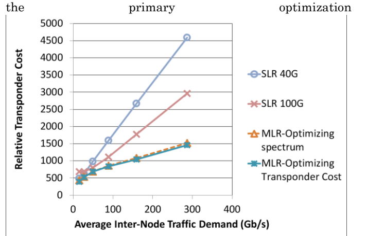
Fig. 3. The relative transponder cost for the fixed-grid networking solutions is presented as a function of the average inter-node traffic demand. Costs are normalized to the value of one 10 Gb/s transponder.
