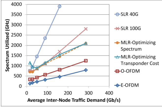
Fig. 1. The spectrum utilization is presented for different networking solutions as a function of the average inter-node traffic demand.
