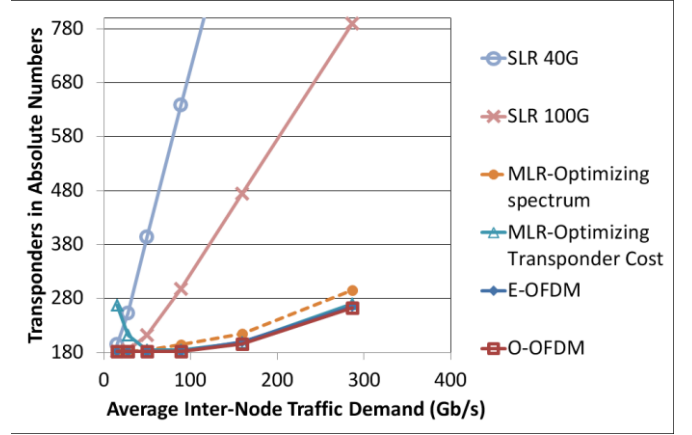
Fig. 2. The required number of transponders is presented for different networking solutions as a function of the average inter-node traffic demand (in absolute numbers).
