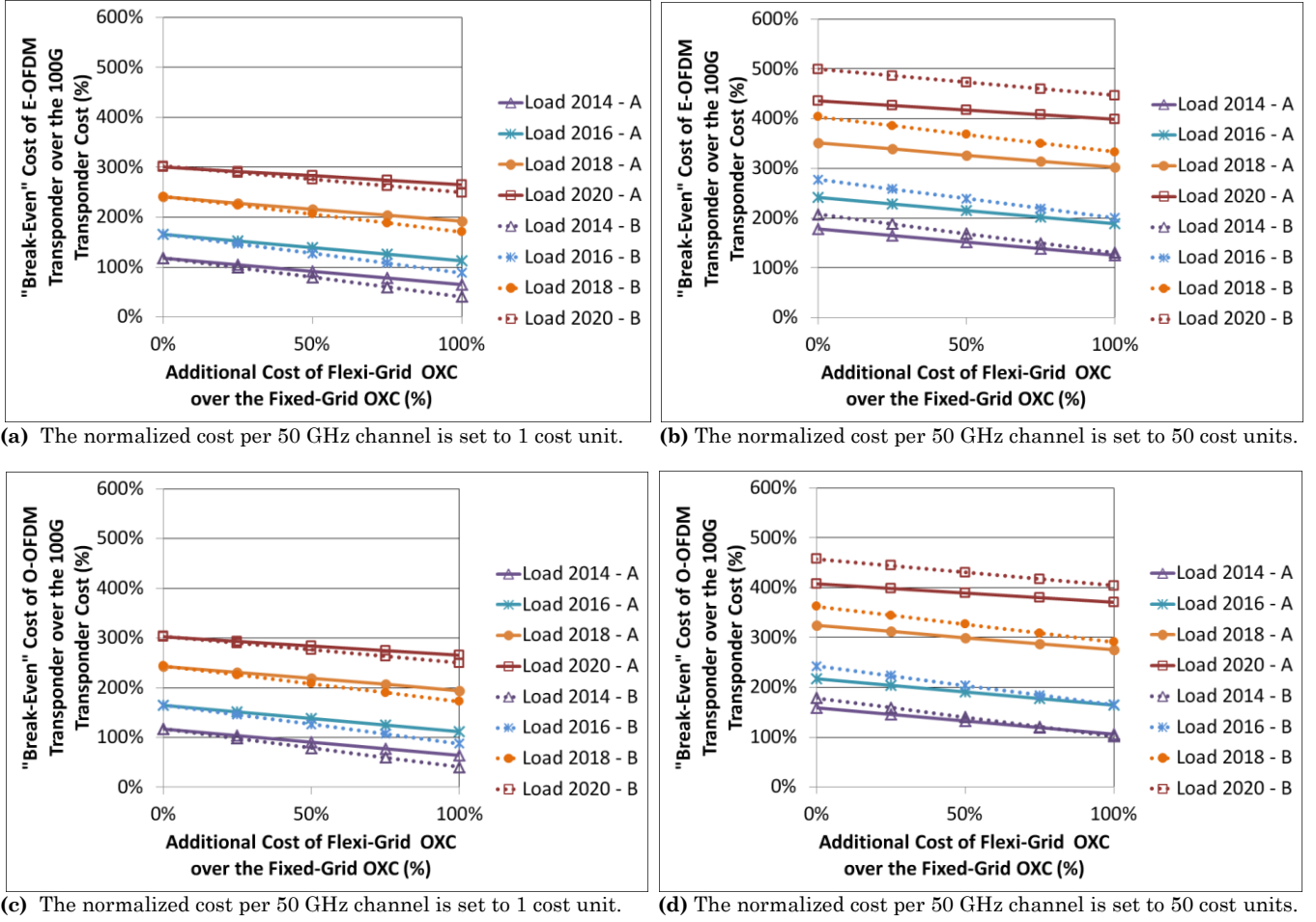
Fig. 5. The “break-even” cost for E-OFDM (a,b) and O-OFDM (c,d) transponders compared to the SLR 100G case is presented as a function of the additional cost of a flex-grid OXC over a fixed-grid OXC - under different traffic loads settings. Options A (solid line) and B (broken line) correspond to a cost value for a 100G transponder of 5.5 and 3.75 cost units, respectively. Reference years 2014 and 2020 have average traffic values of approximately 50 Gb/s and 300 Gb/s respectively. An annual growth rate of 34% is assumed for the traffic demand.
