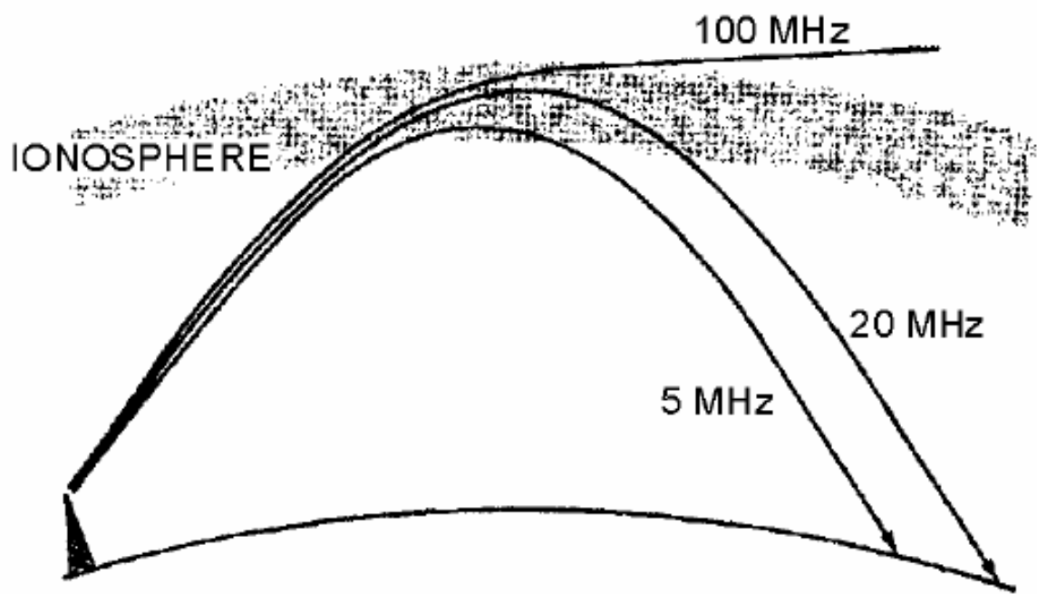
Figure 2-16.—Frequency versus refraction and distance.
