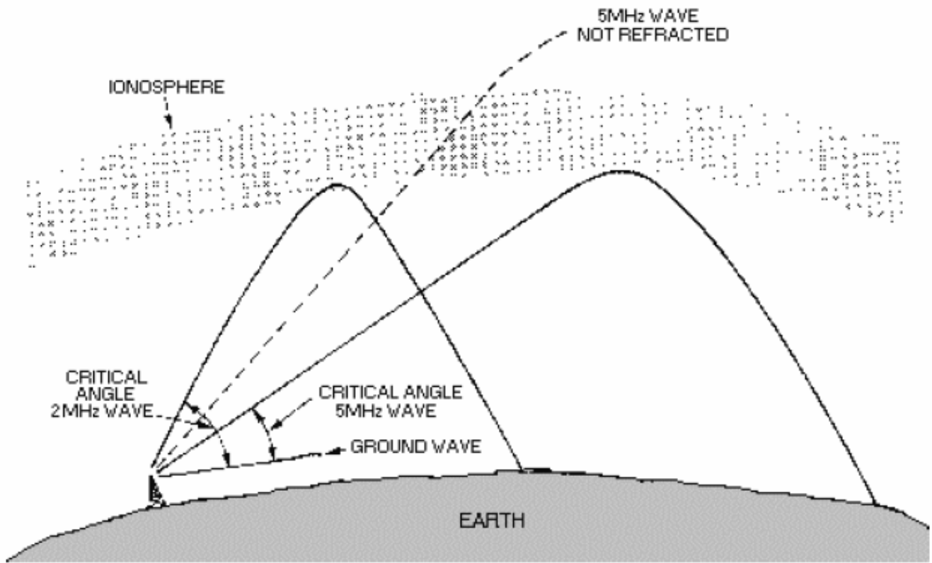
Figure 2-18.—Effects of frequency on the critical angle.
