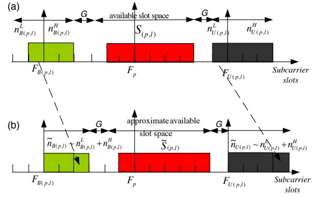
Fig. 3. (a) Upper and lower spectrum-adjacent connections following the DHL policy, (b) approximate system DHL where the bottom and upper spectrum-adjacent connections use only their higher spectrum slots.
