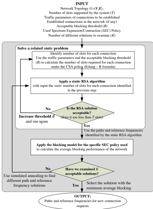
Fig. 5. Block diagram of the proposed RSA algorithm to assign paths and reference frequencies to a set of time-varying connection requests.
