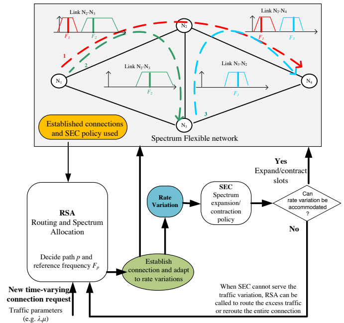
Fig. 1. Flow diagram for serving a connection request. RSA is used to determine the path and reference frequency and SEC policy takes care of traffic variations. When the SEC policy cannot accommodate a traffic variation, or if the rate exceeds the capability of the transponder, RSA can be triggered to set up an additional connection or reroute the existing connection.
