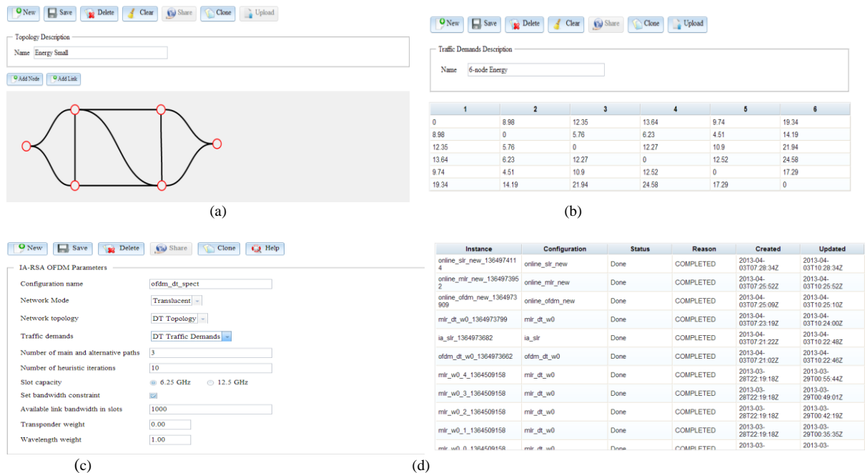
Figure 2. (a) create network topology (b) define traffic requests (c) create configuration (d) information for all instances
