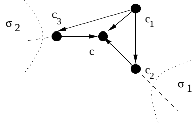
Figure 3.8: A configuration of the effective neighborhood of an optimal call c .
