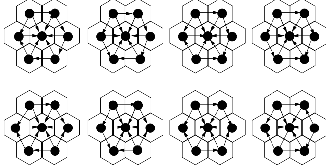
Figure 3.5: The case |\gamma| = 6 .
