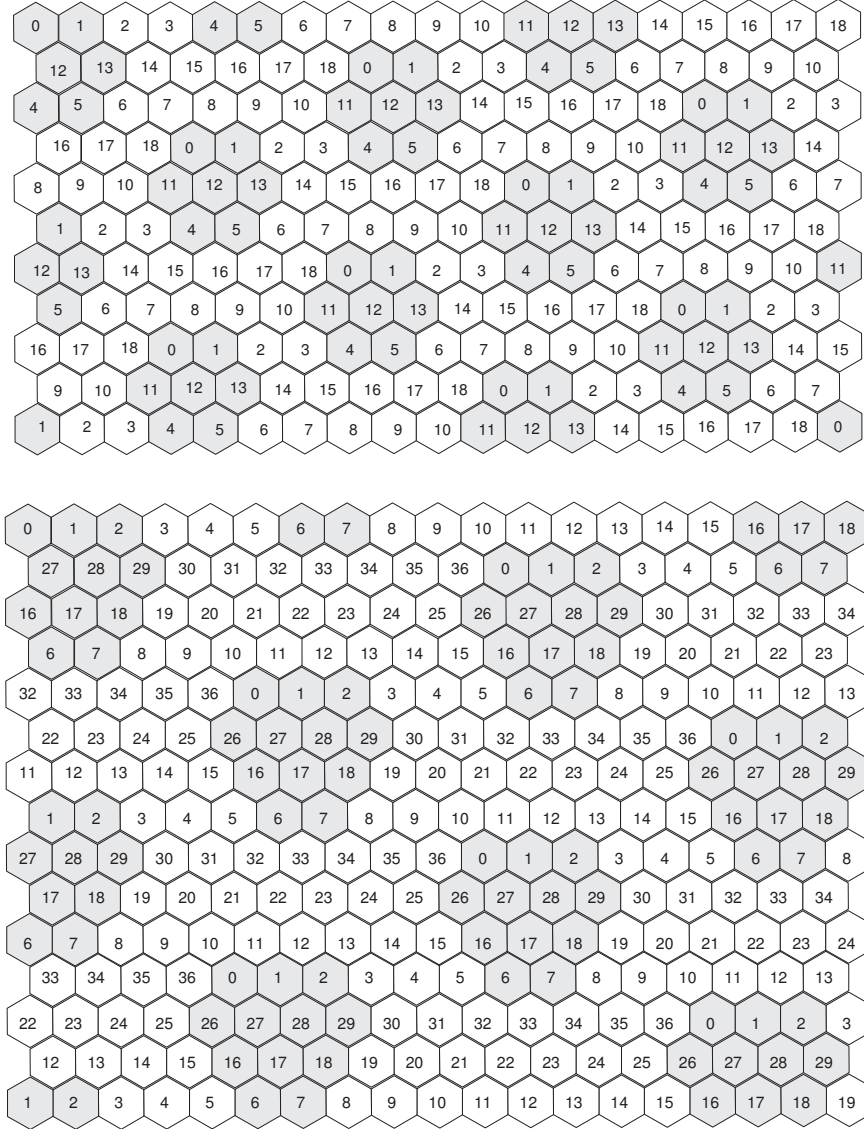
Figure 3.12: Examples of the colorings used by the algorithms CRS-3 and CRS-4. The skewed cells are those colored with the colors in set s_0 .
