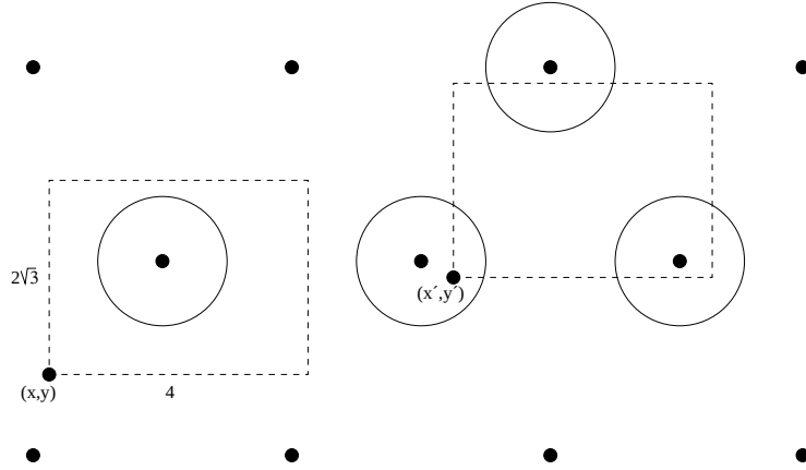
Figure 4.5: Disk centers (x, y) and (x', y') and the rectangles where points (x + \alpha, y + \beta) and (x' + \alpha, y' + \beta) are uniformly distributed.
